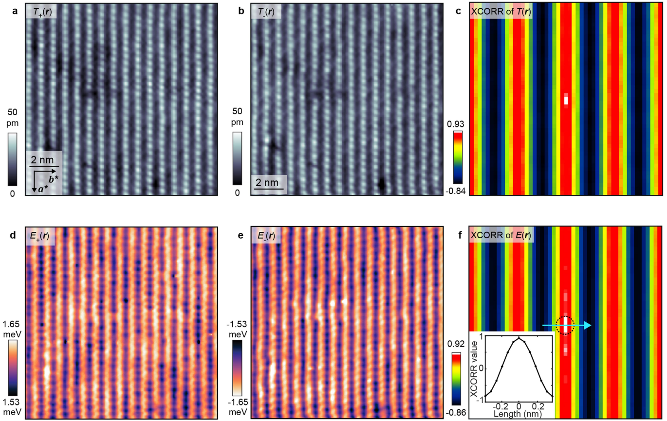
Extended Data Fig. 5 | Spatial registration of topographs and gap maps. a, b , 12 nm \times 12 nm topographs after registration. These topographs were obtained concomitantly as dI/dV|_{SIS}(r, V) maps recording positive and negative coherence peaks, respectively. c , XCORR map of the registered topographs. The correlation coefficient is 0.93, indicating that the two topographs are almost identical. The maxima of the XCORR map is a single pixel wide, which suggests a registration precision of 0.5 pixels, equivalent to registration
