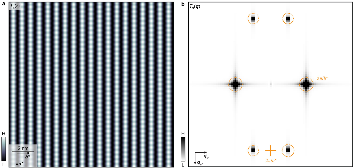
Extended Data Fig. 2 | Simulated topography of UTe_2 and its Fourier transform. a , Simulated topograph, T_s(r) of the (0-11) cleave surface of UTe_2 . b , Fourier transform of simulated topograph, T_s(q) . The six primary peaks occur at the reciprocal-lattice wavevectors and are observed in the experimental STM data.
